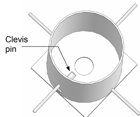
FIG. 5B: Top view of sleeve
