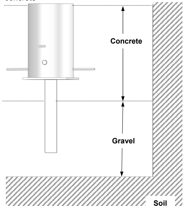
FIG. 3: Prepare the ground and fix the sleeve in concrete
